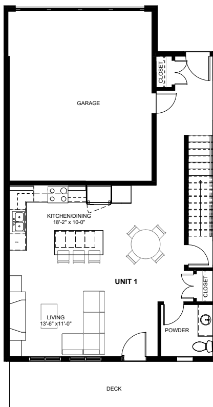
Unit 1 & 4 - Main Floor
