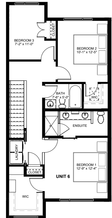
Unit 6 - Third Floor
