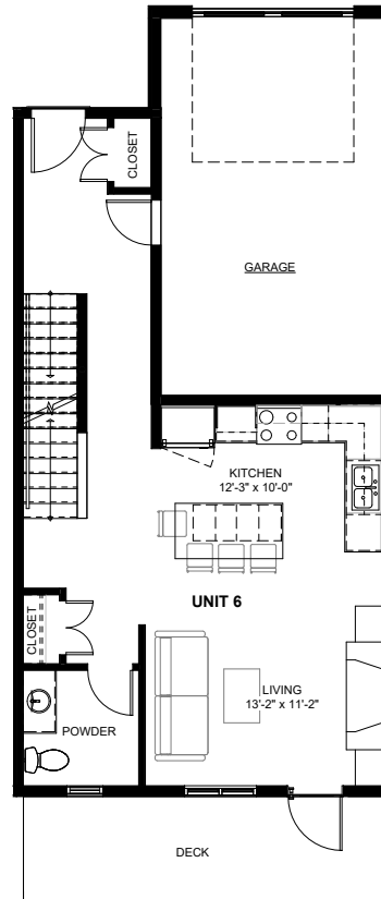
Unit 6 - Main Floor
